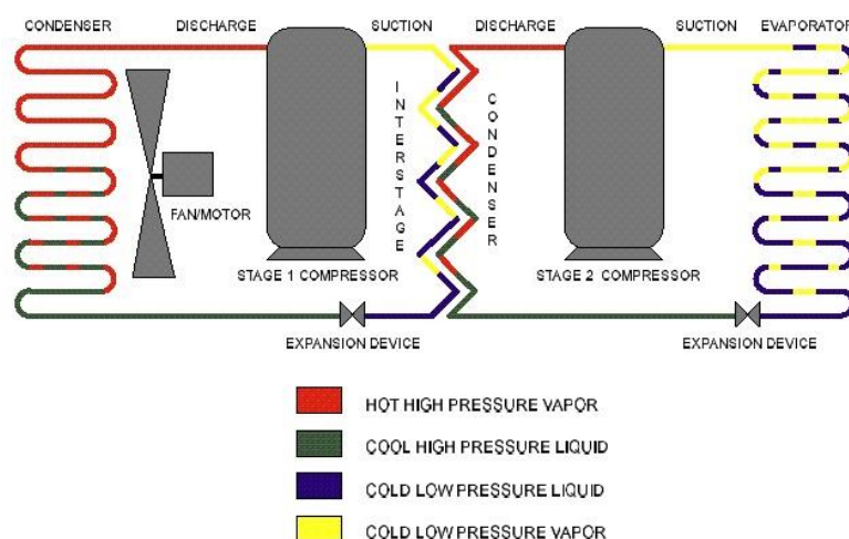
Flow Schematic
